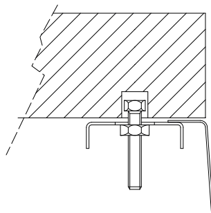
lateral section
